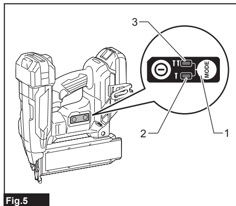
Fig.5 ► 1. Actuation mode switch button 2. Sequential actuation mode 3. Contact actuation mode
